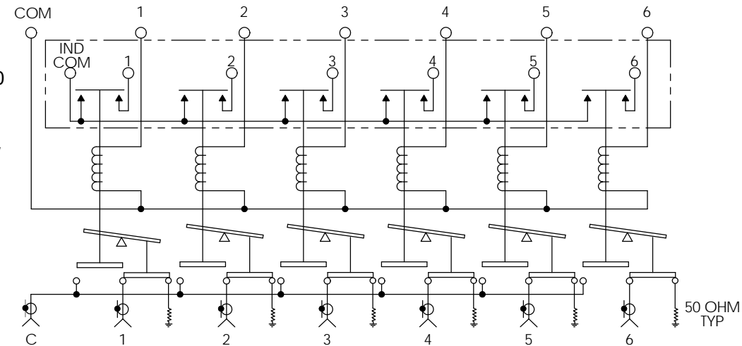
SCHMATIC DIAGRAM SHOWN IN NORMALLY OPEN POSITION (DE-ENERGIZED)
