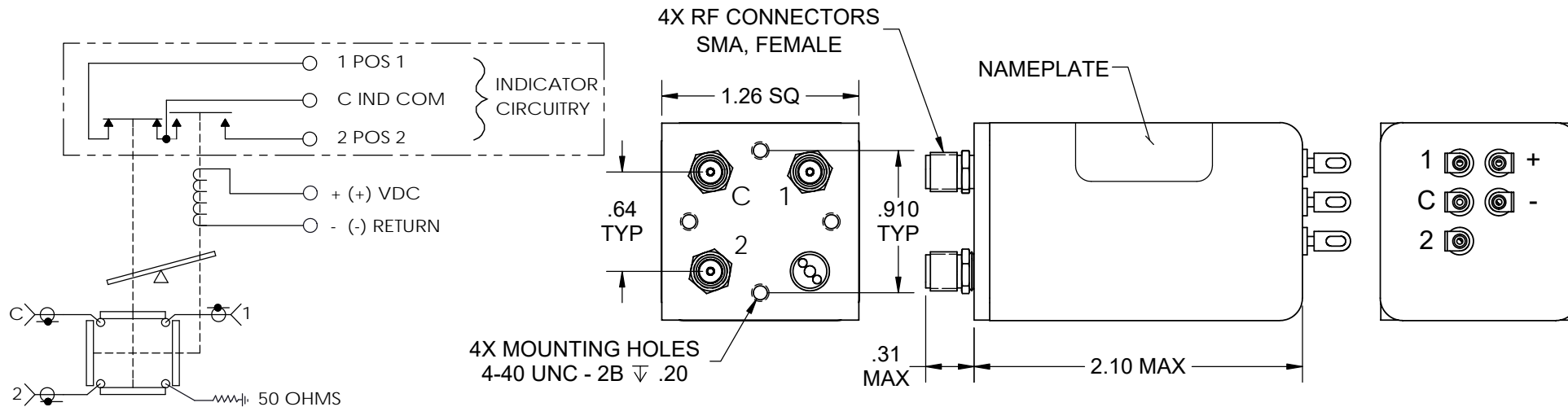
SCHEMATIC DIAGRAM SHOWN IN FAILSAFE POSITION 1
