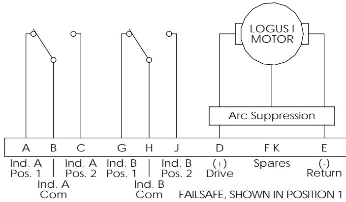
Electrical Circuit B, Connector MS3112E-12-10P
