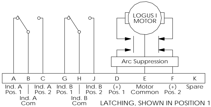
Electrical Circuit B, Connector MS3112E-12-10P
