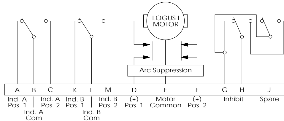
Electrical Circuit J, Connector MS3112E-12-10P
