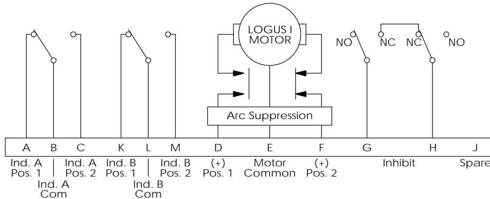
Electrical Circuit B w/TTL, Connector MS3112E-12-10P
