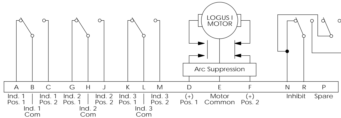
Electrical Circuit G, Connector MS3112E-14-15P
