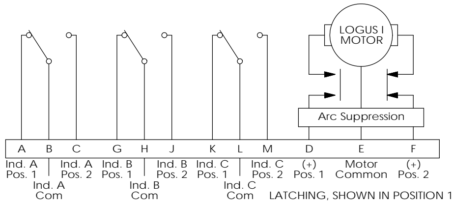
Electrical Circuit C, Connector MS3112E-14-15P
