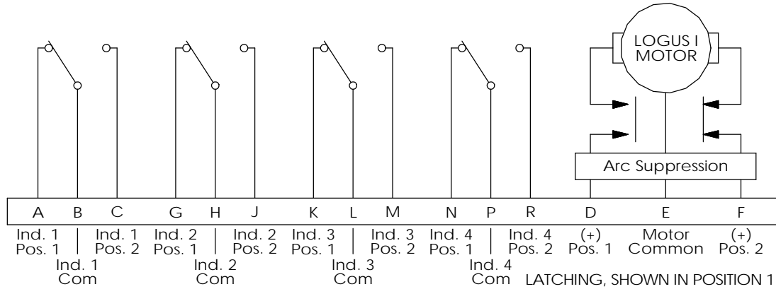
Electrical Circuit D, Connector MS3112E-14-15P
